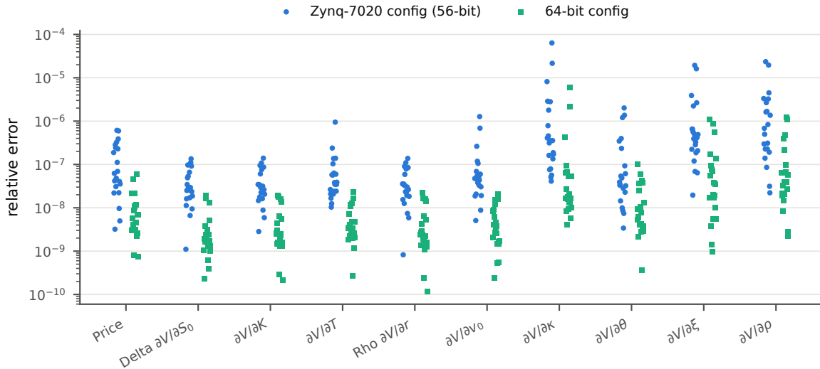
Generated shared-multiplier datapaths vs double-precision COS, 21 parameter sets
